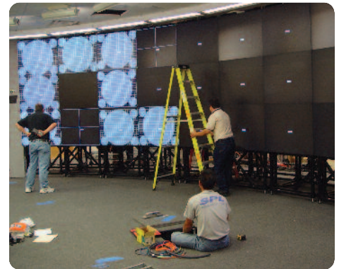
In the awe-inspiring curved main video wall, a support structure holding 27 screen modules—a 9-wide by 3-high array of Christie Digital Reflex II Screen Can Assemblies—is lit up by 27 Christie Digital RPMS-500xe DLP projectors.
